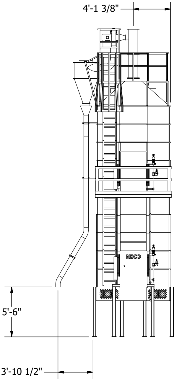
FRONT ELEVATION VIEW SCALE 1 / 75
