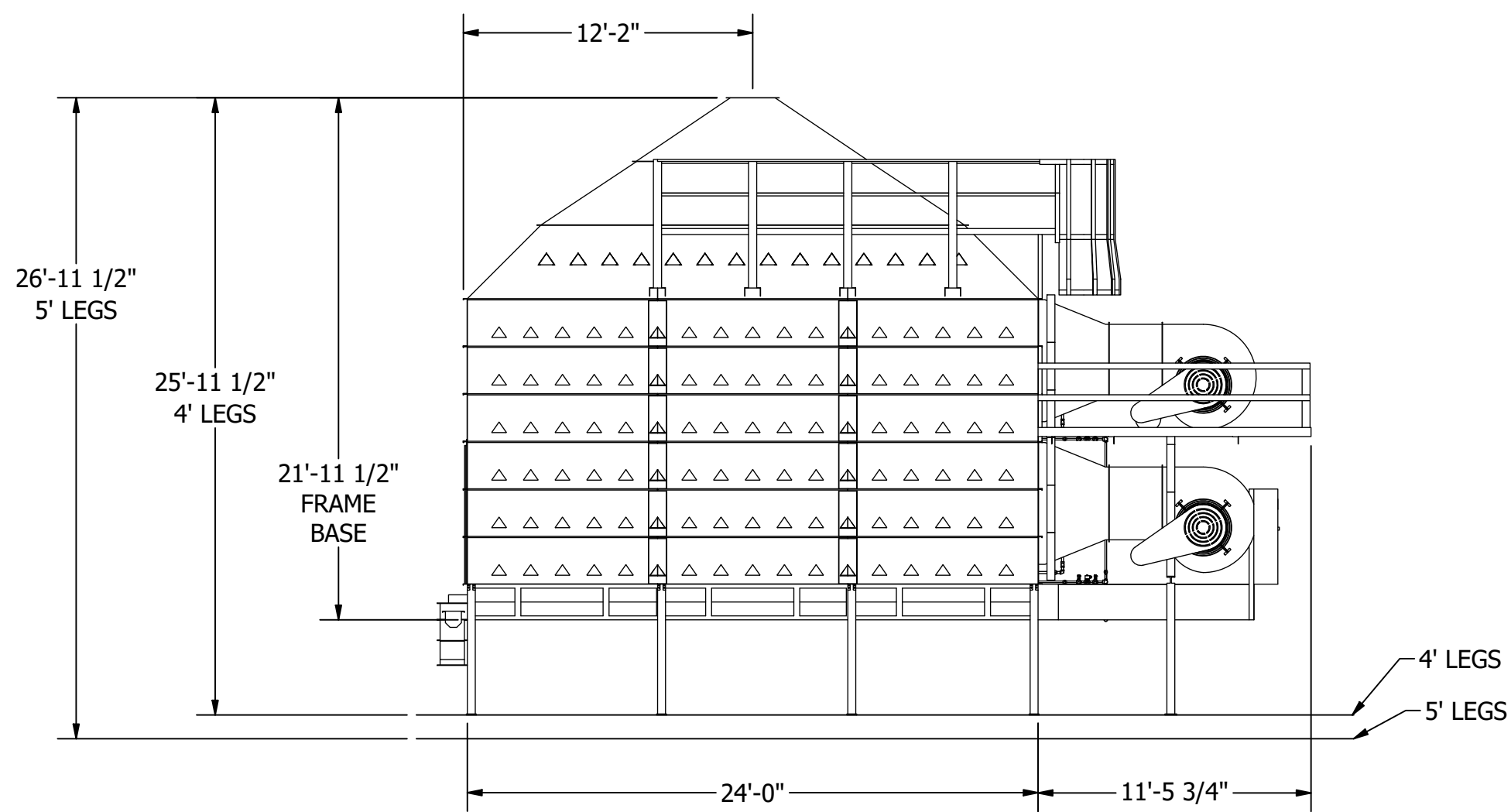
SIDE ELEVATION VIEW SCALE 1 / 75
