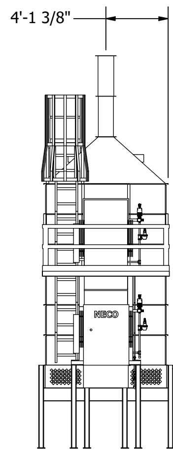
FRONT ELEVATION VIEW SCALE 1 / 75
